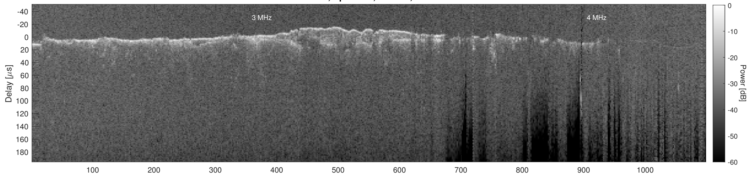
Orbit 10783, Cluttergram
