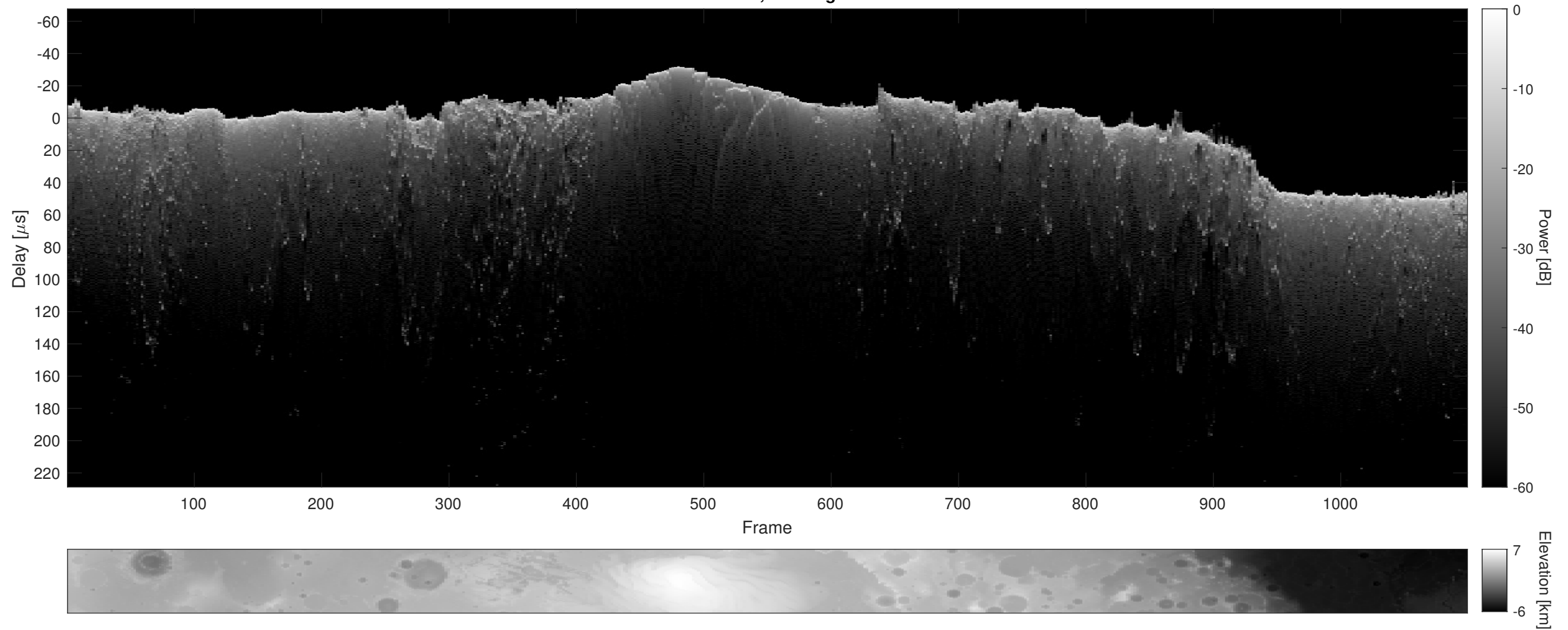
Orbit 10784, Cluttergram
