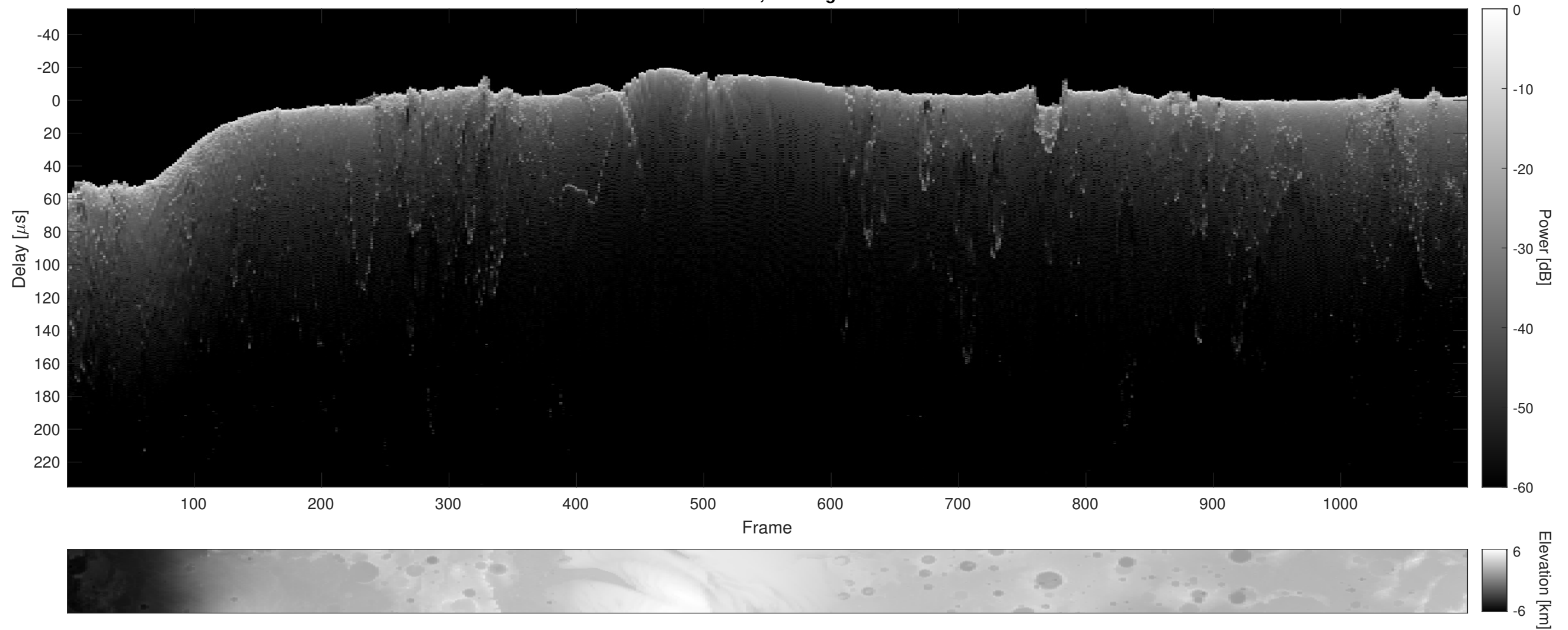
Orbit 10786, Cluttergram
