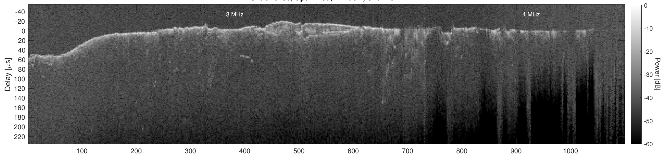
Orbit 10786, Cluttergram
