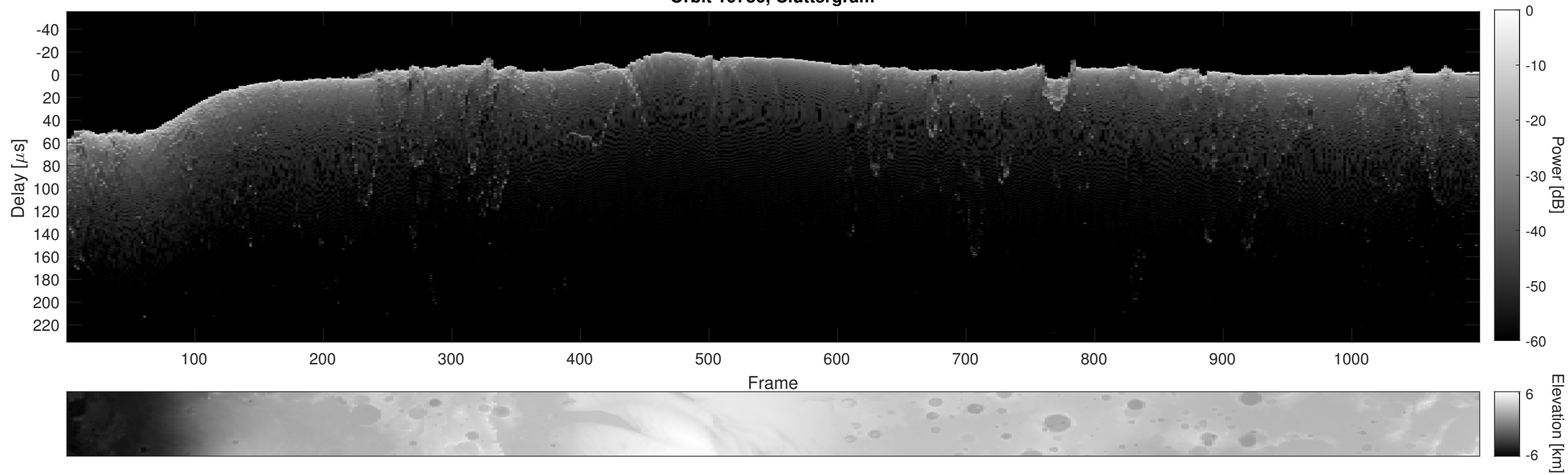
Orbit 10786, Cluttergram
