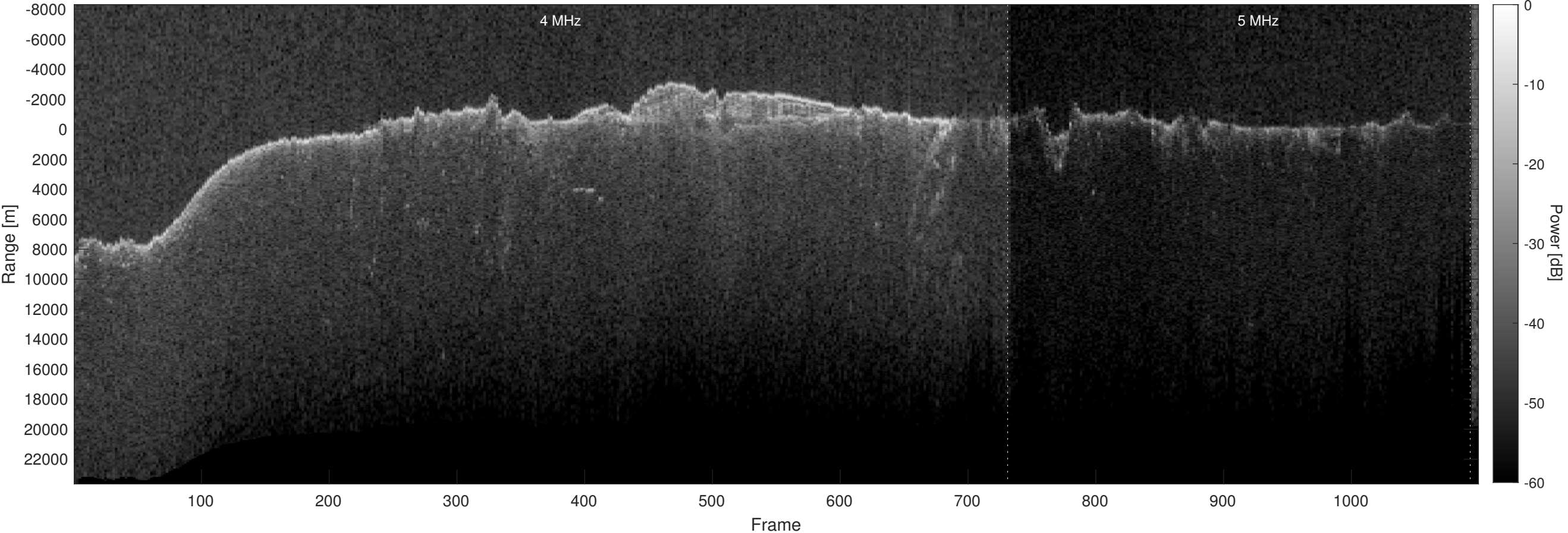
Orbit 10786, Optimized, Window, Depth-Corrected, Channel 2
