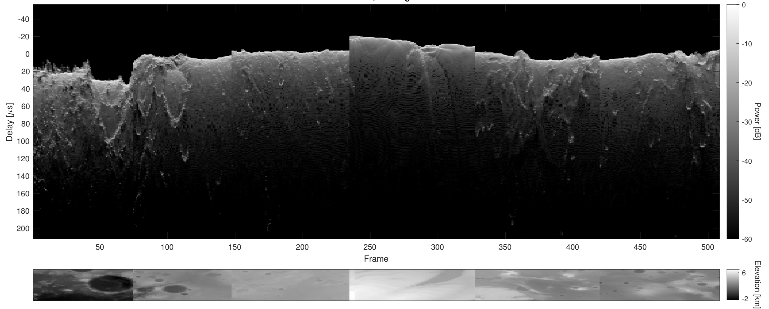
Orbit 10787, Cluttergram
