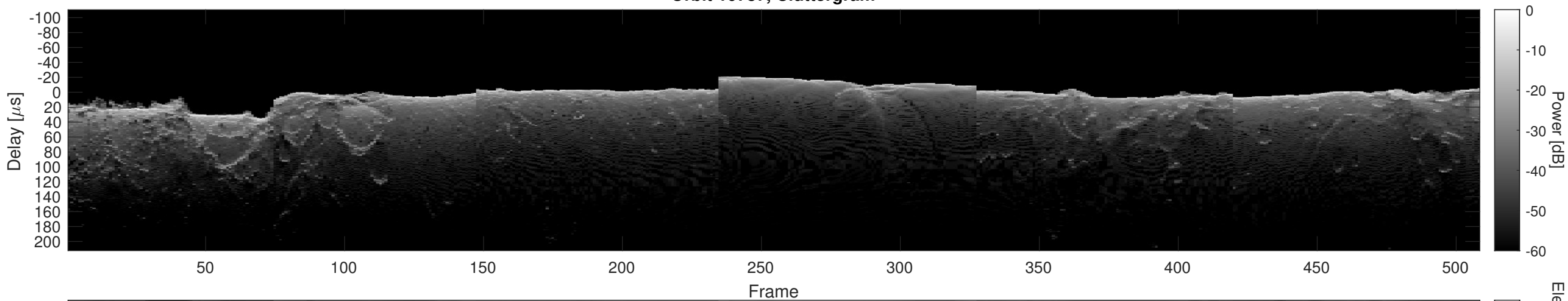
Orbit 10787, Cluttergram
