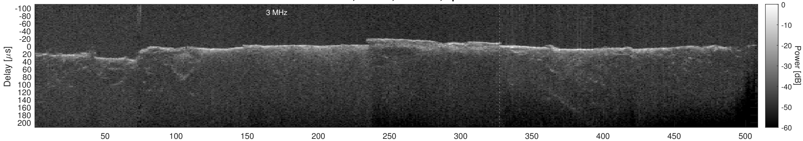
Orbit 10787, Cluttergram
