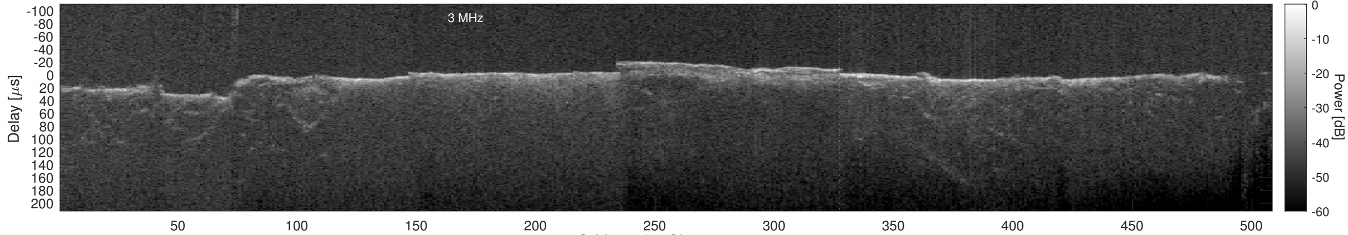
Orbit 10787, Cluttergram
