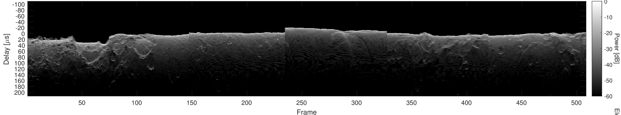
Orbit 10787, Cluttergram
