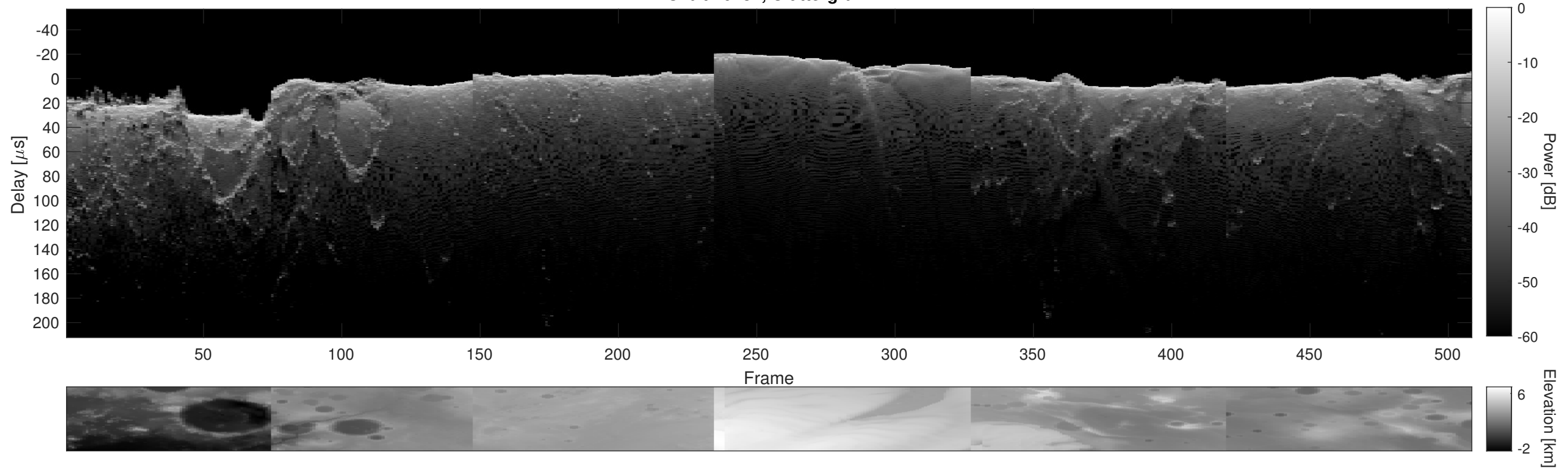
Orbit 10787, Cluttergram
