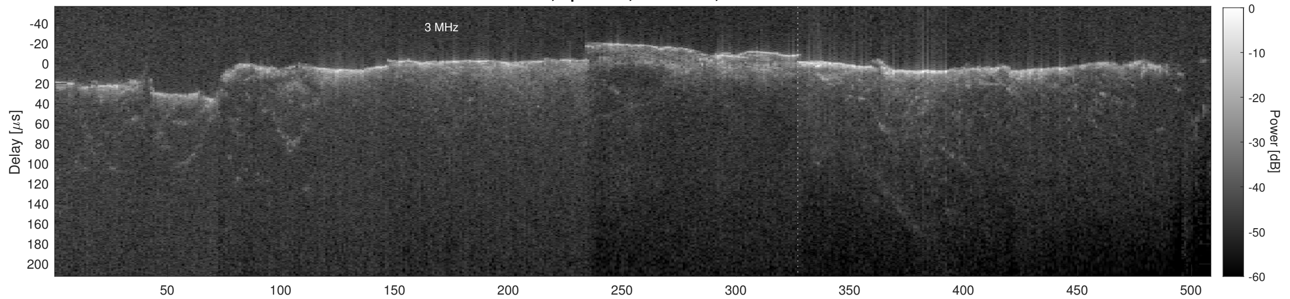
Orbit 10787, Cluttergram
