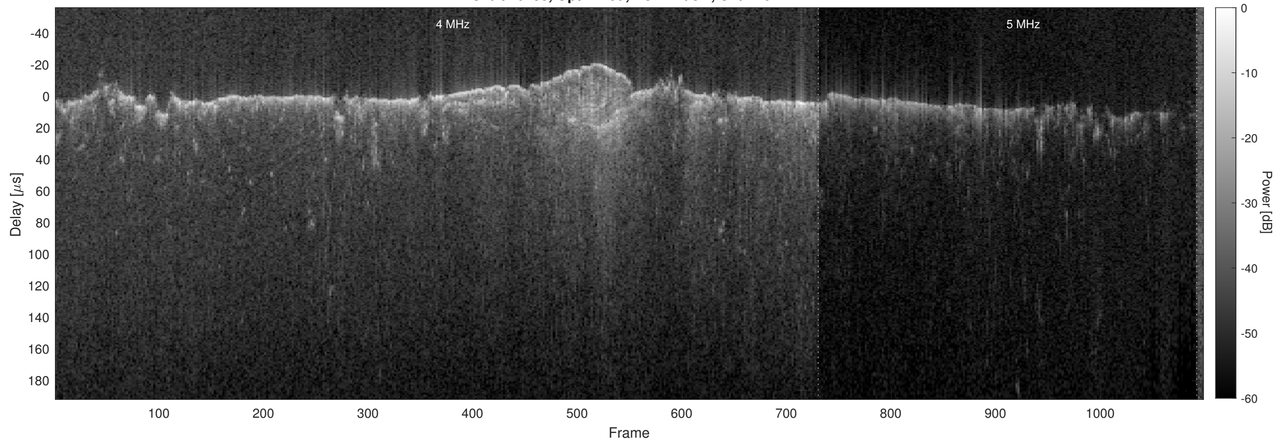
Orbit 10788, Optimized, No Window, Channel 2
