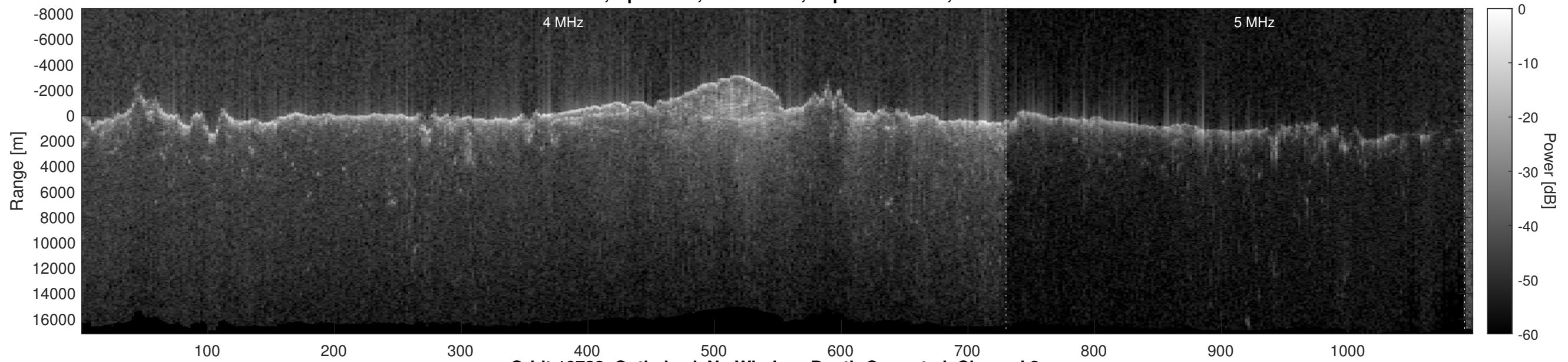
Orbit 10788, Optimized, No Window, Depth-Corrected, Channel 2
