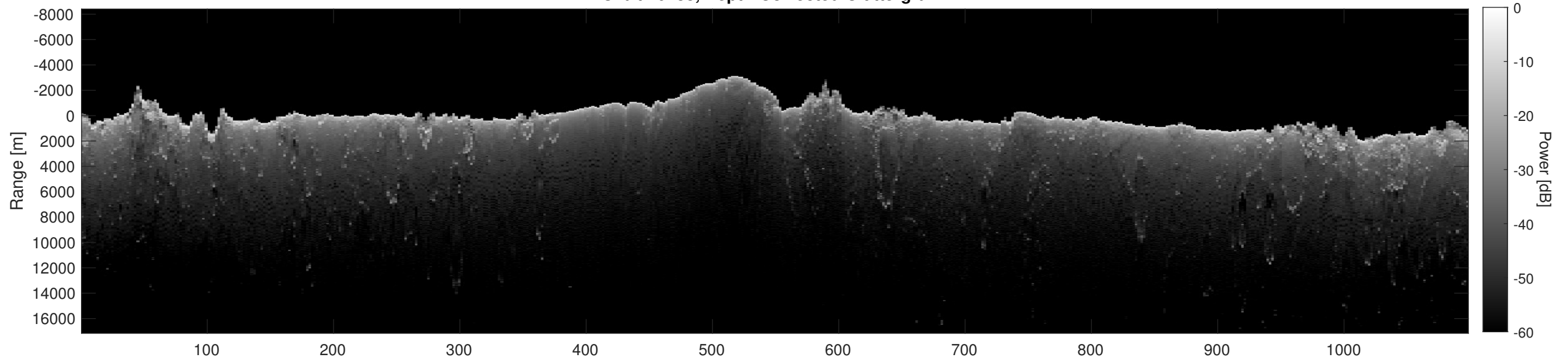
Orbit 10788, Depth-Corrected Cluttergram
