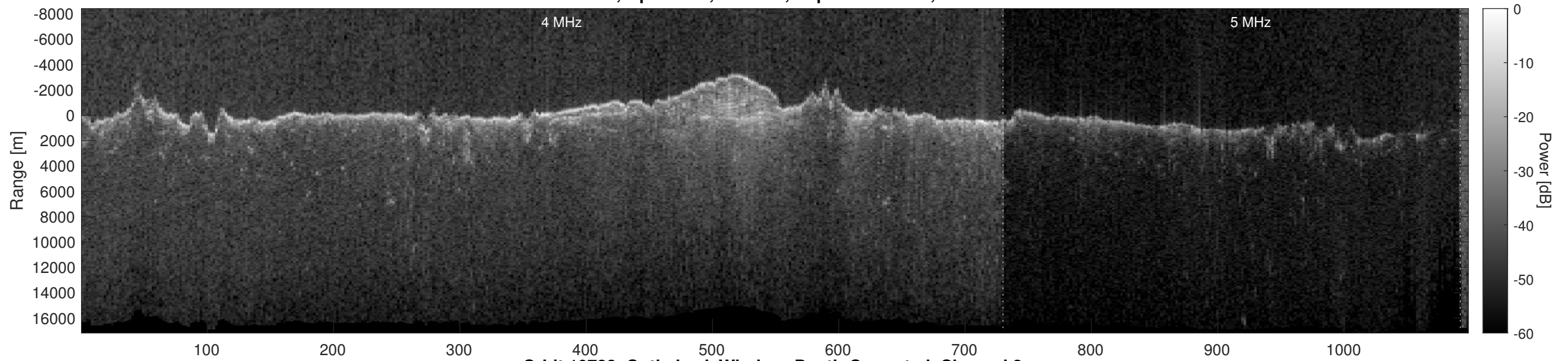
Orbit 10788, Optimized, Window, Depth-Corrected, Channel 2
