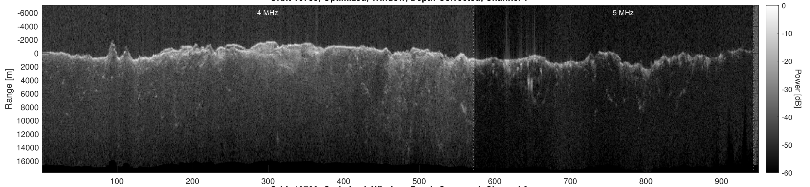
Orbit 10789, Optimized, Window, Depth-Corrected, Channel 2
