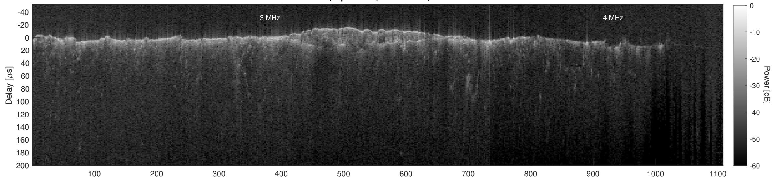
Orbit 10790, Cluttergram
