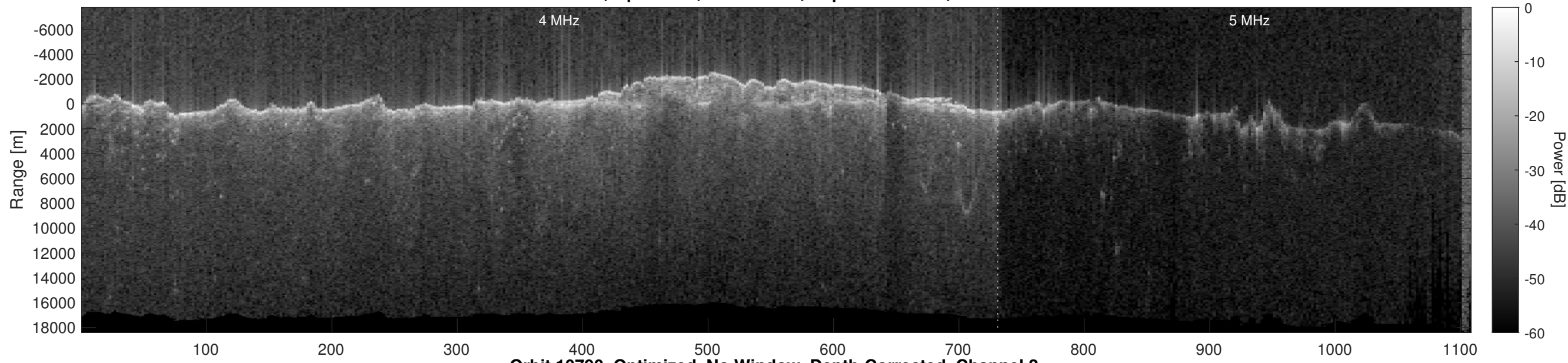
Orbit 10790, Optimized, No Window, Depth-Corrected, Channel 2
