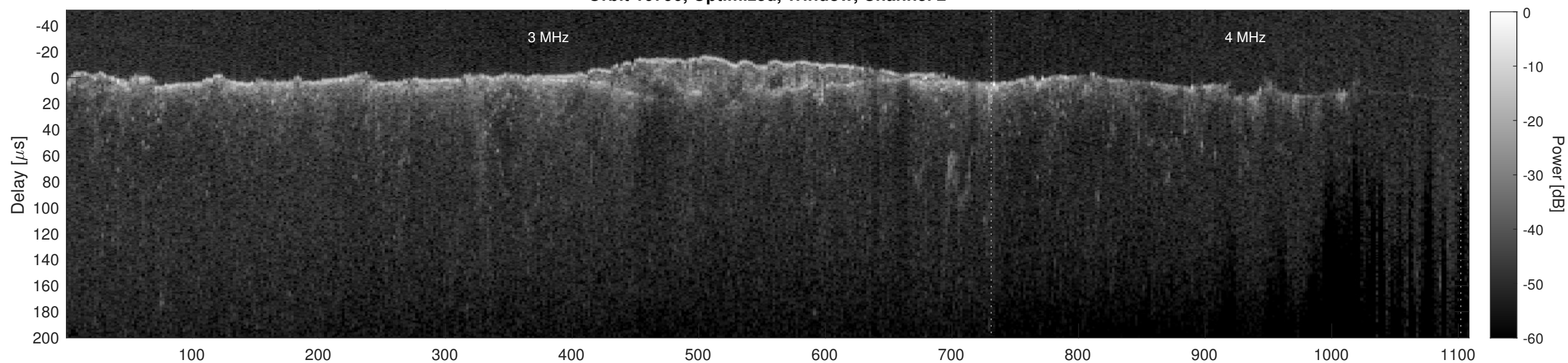
Orbit 10790, Cluttergram
