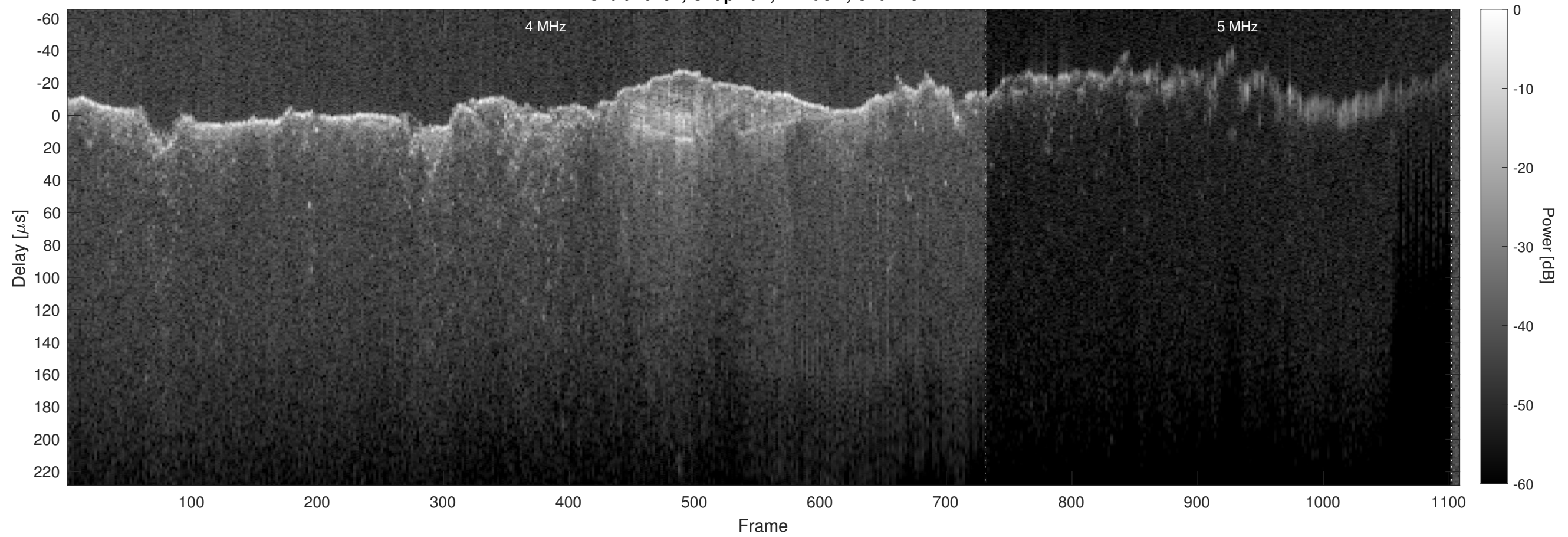
Orbit 10791, Chapman, Window, Channel 2
