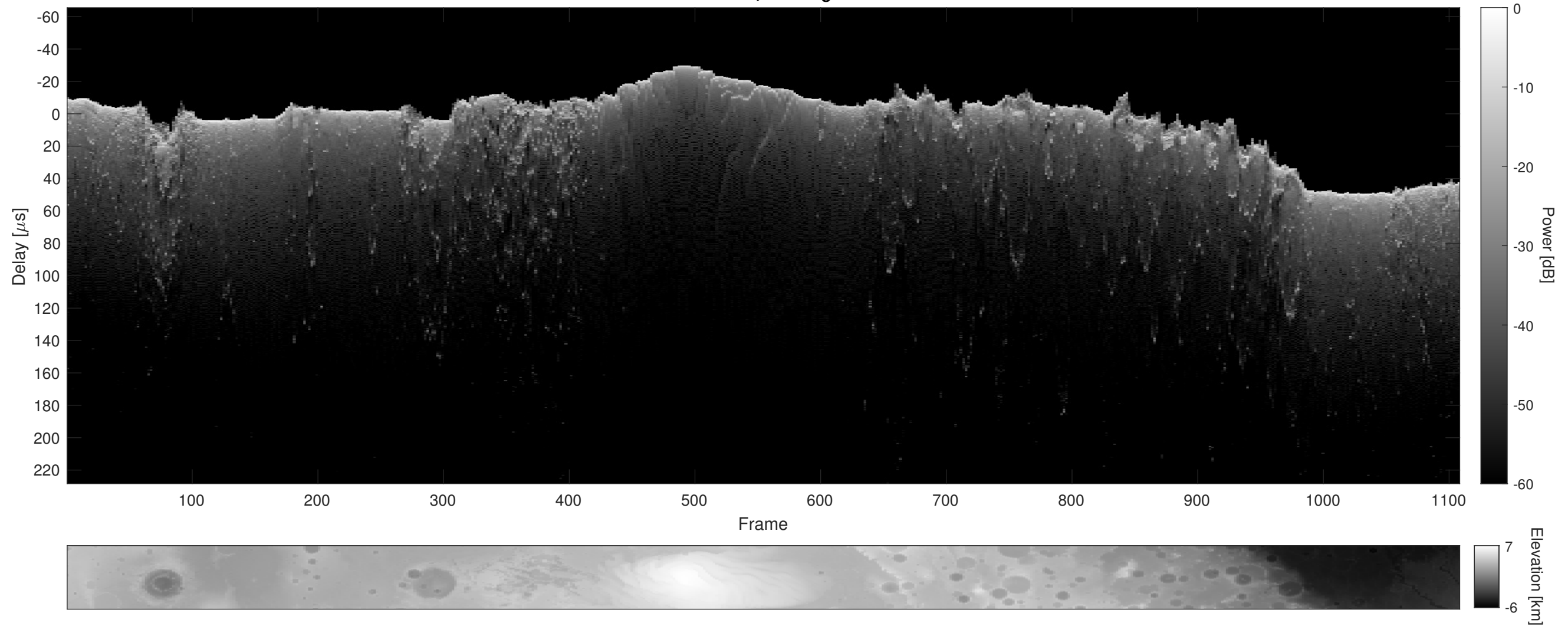
Orbit 10791, Cluttergram
