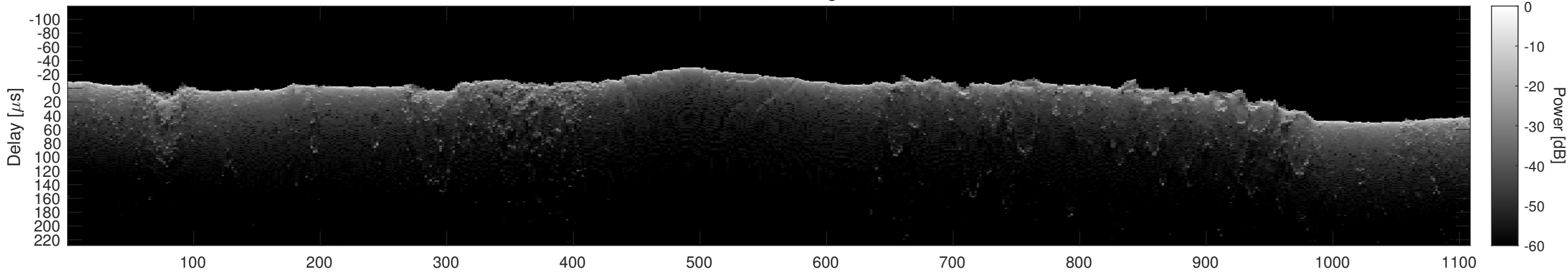
Orbit 10791, Cluttergram
