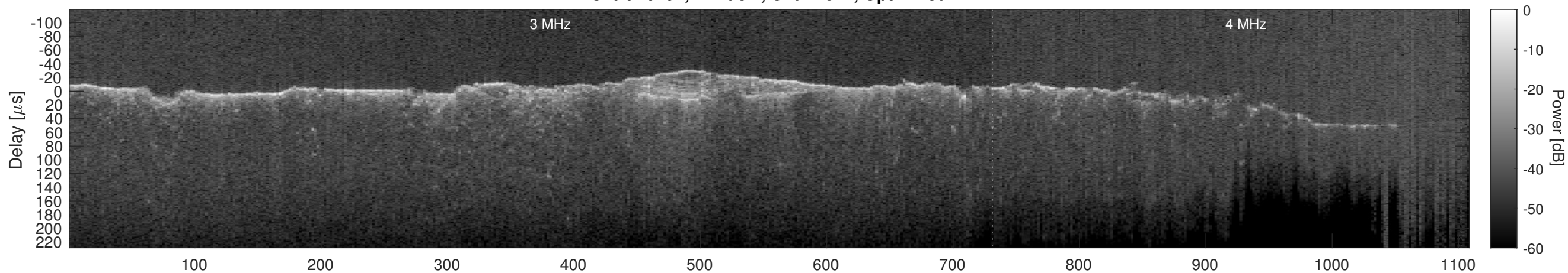
Orbit 10791, Cluttergram
