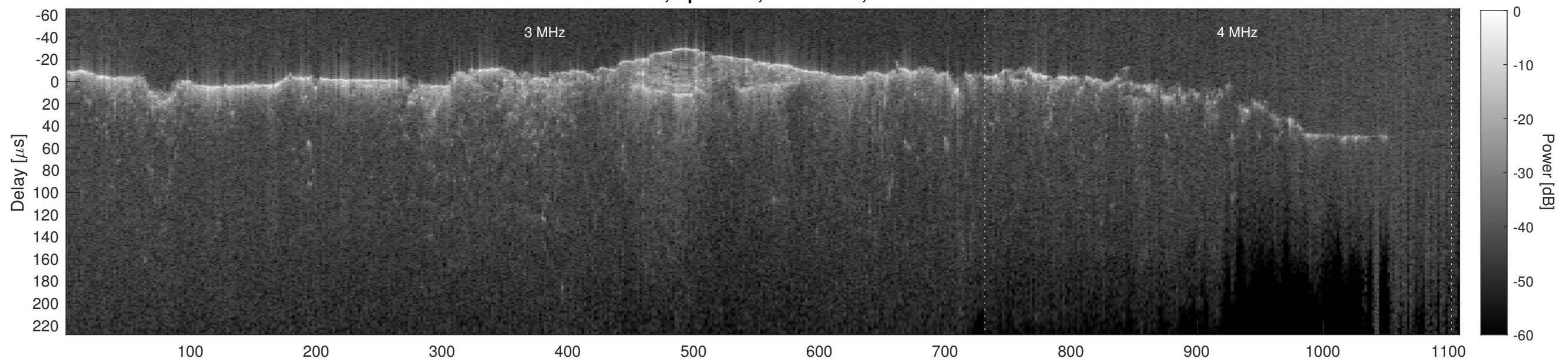
Orbit 10791, Cluttergram
