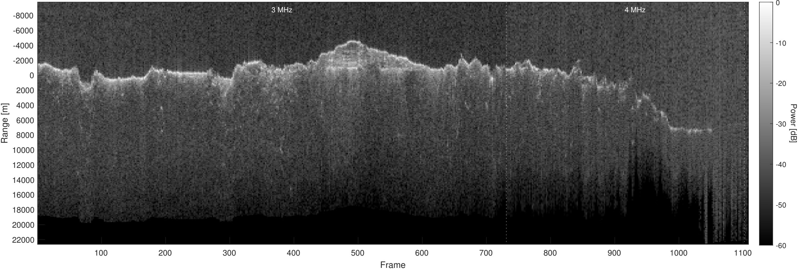
Orbit 10791, Optimized, Window, Depth-Corrected, Channel 2
