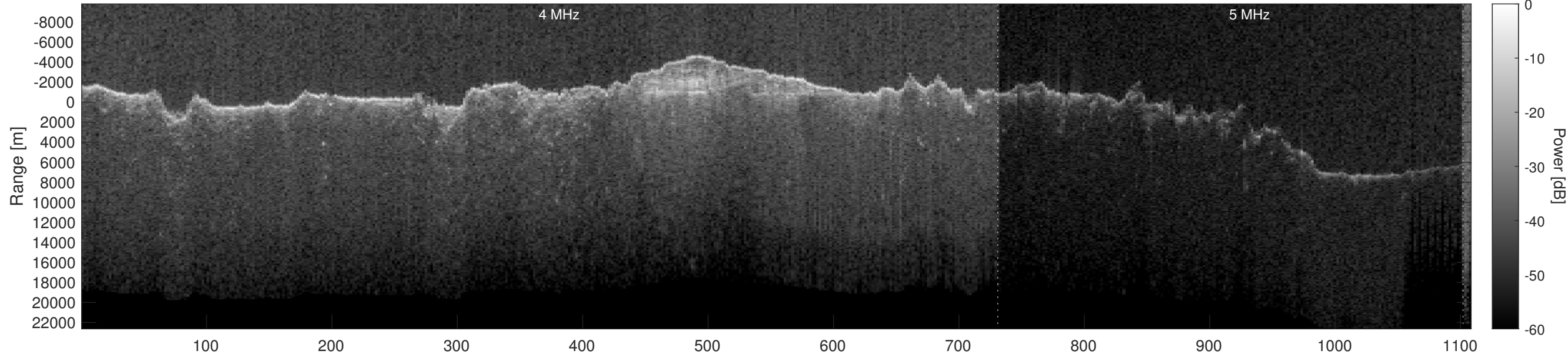
Orbit 10791, Optimized, Window, Depth-Corrected, Channel 2
