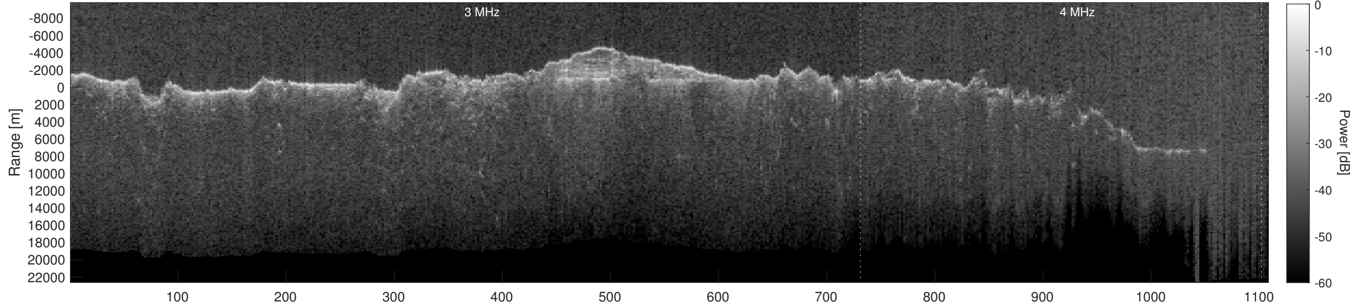
Orbit 10791, Depth-Corrected Cluttergram
