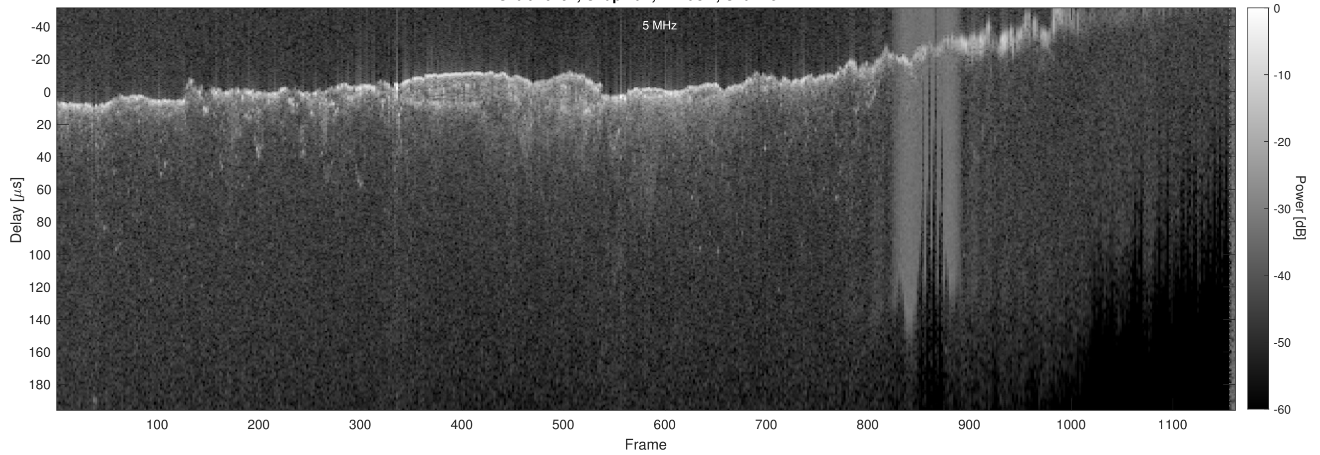
Orbit 10792, Chapman, Window, Channel 2
