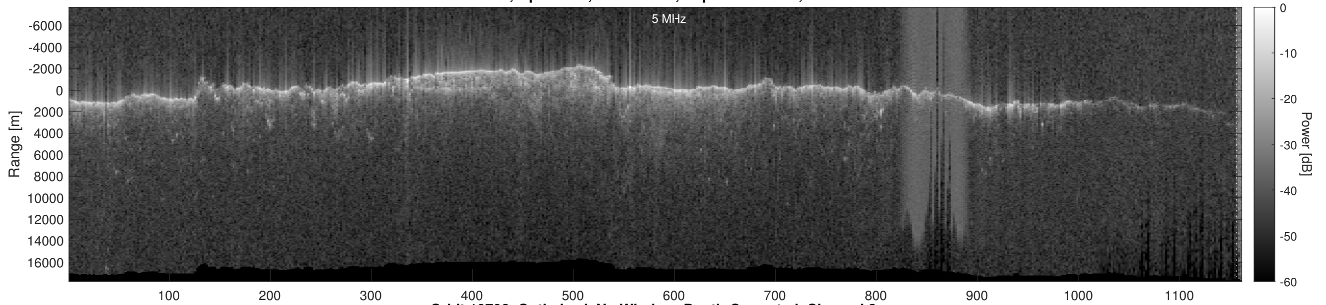
Orbit 10792, Optimized, No Window, Depth-Corrected, Channel 2
