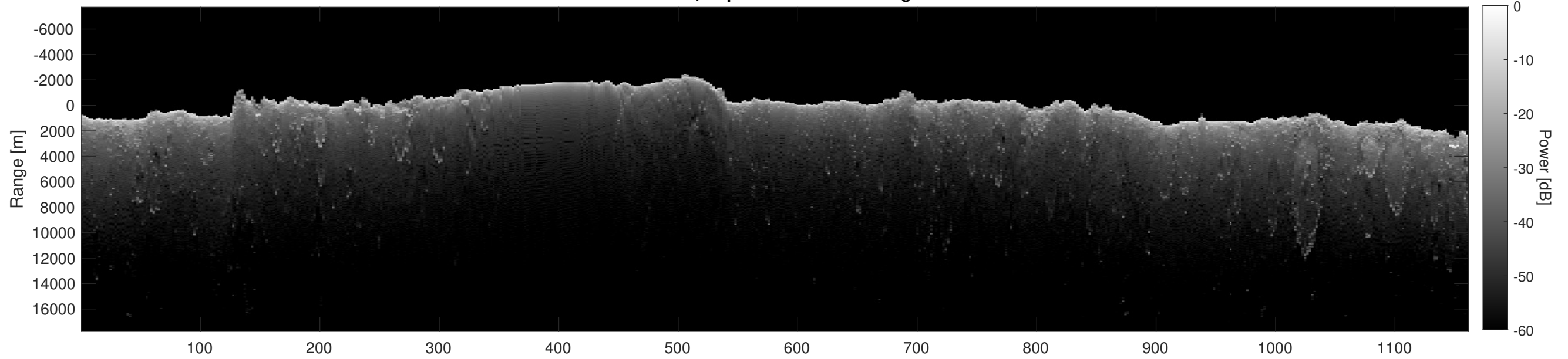
Orbit 10792, Depth-Corrected Cluttergram
