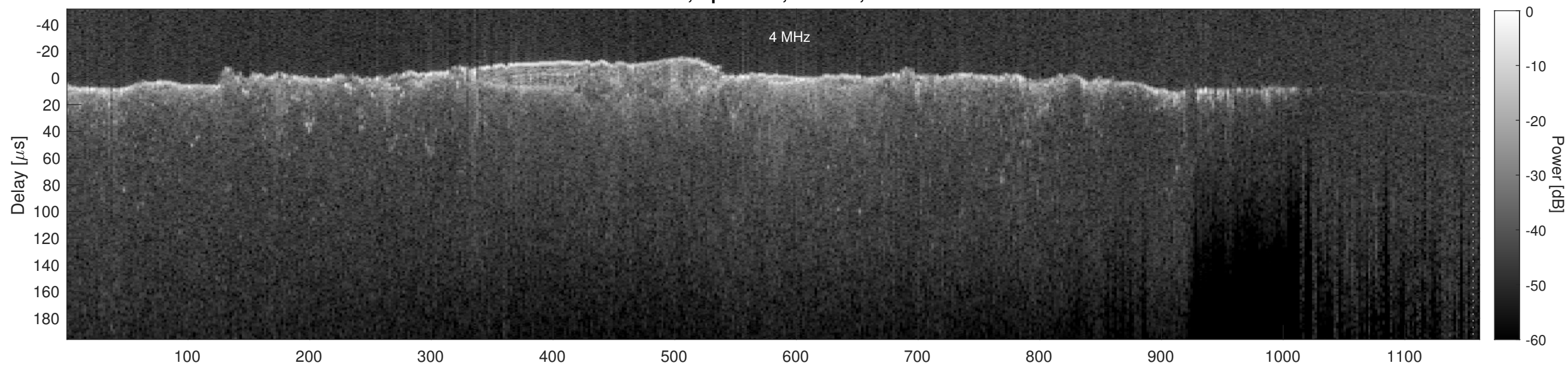
Orbit 10792, Cluttergram
