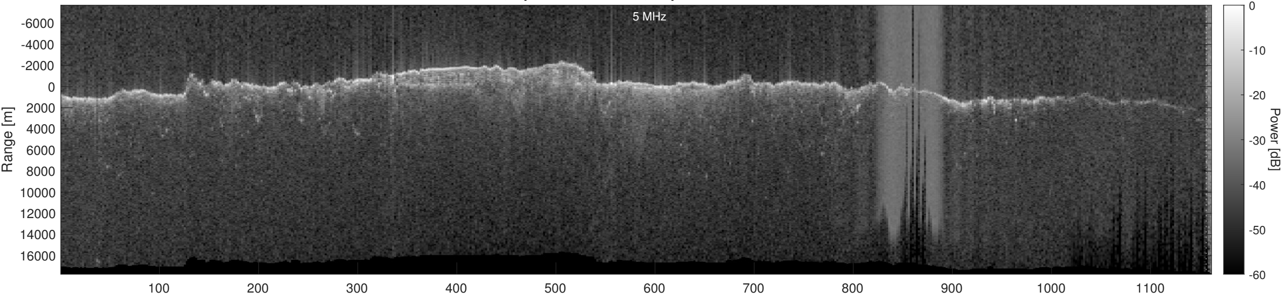
Orbit 10792, Optimized, Window, Depth-Corrected, Channel 2
