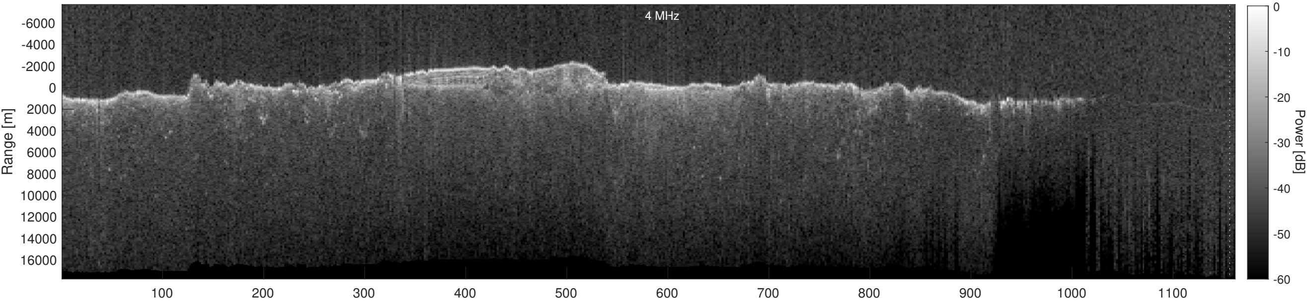
Orbit 10792, Depth-Corrected Cluttergram
