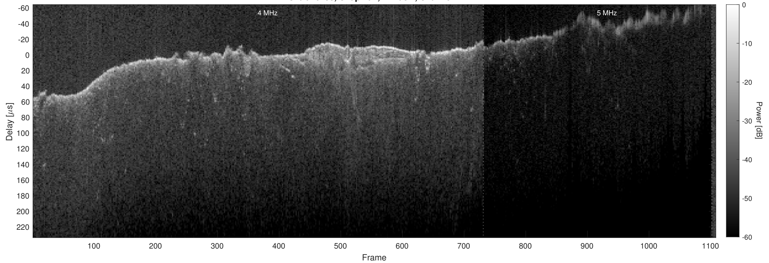
Orbit 10793, Chapman, Window, Channel 2
