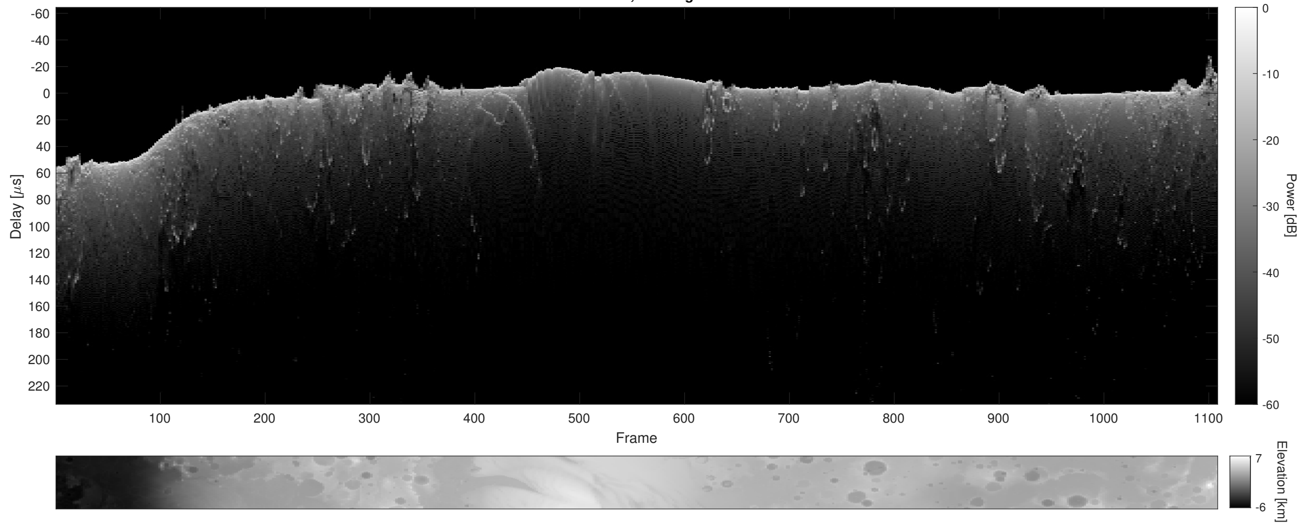
Orbit 10793, Cluttergram
