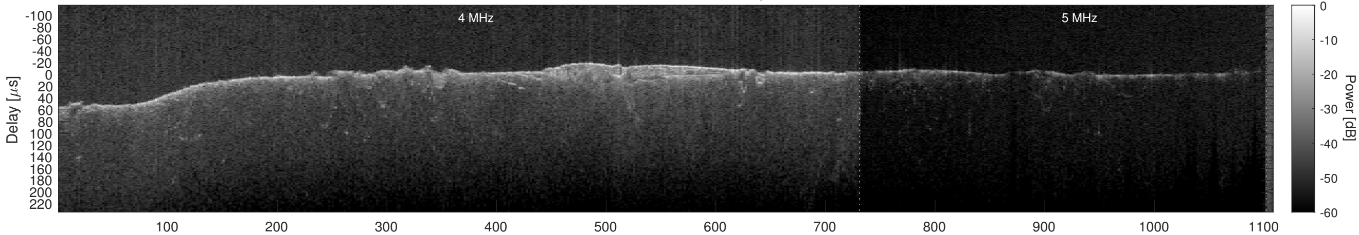
Orbit 10793, Cluttergram
