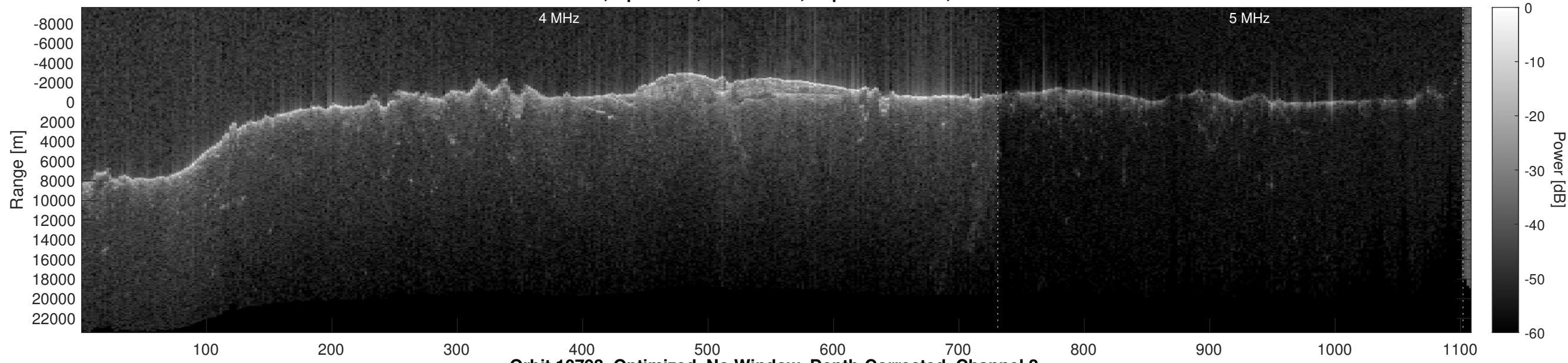
Orbit 10793, Optimized, No Window, Depth-Corrected, Channel 2
