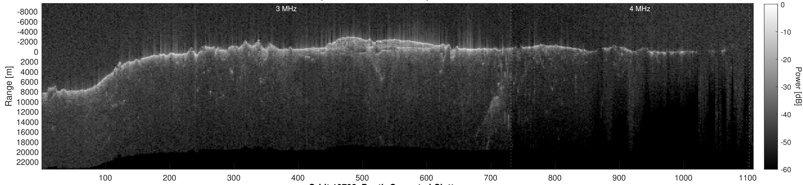
Orbit 10793, Depth-Corrected Cluttergram
