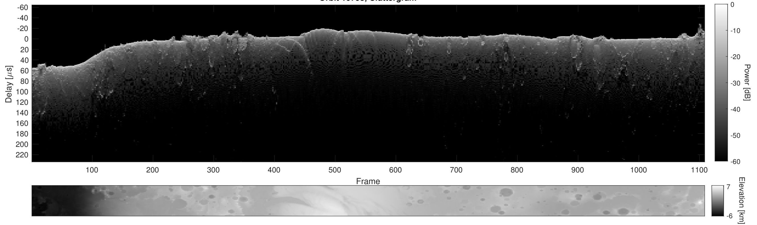
Orbit 10793, Cluttergram
