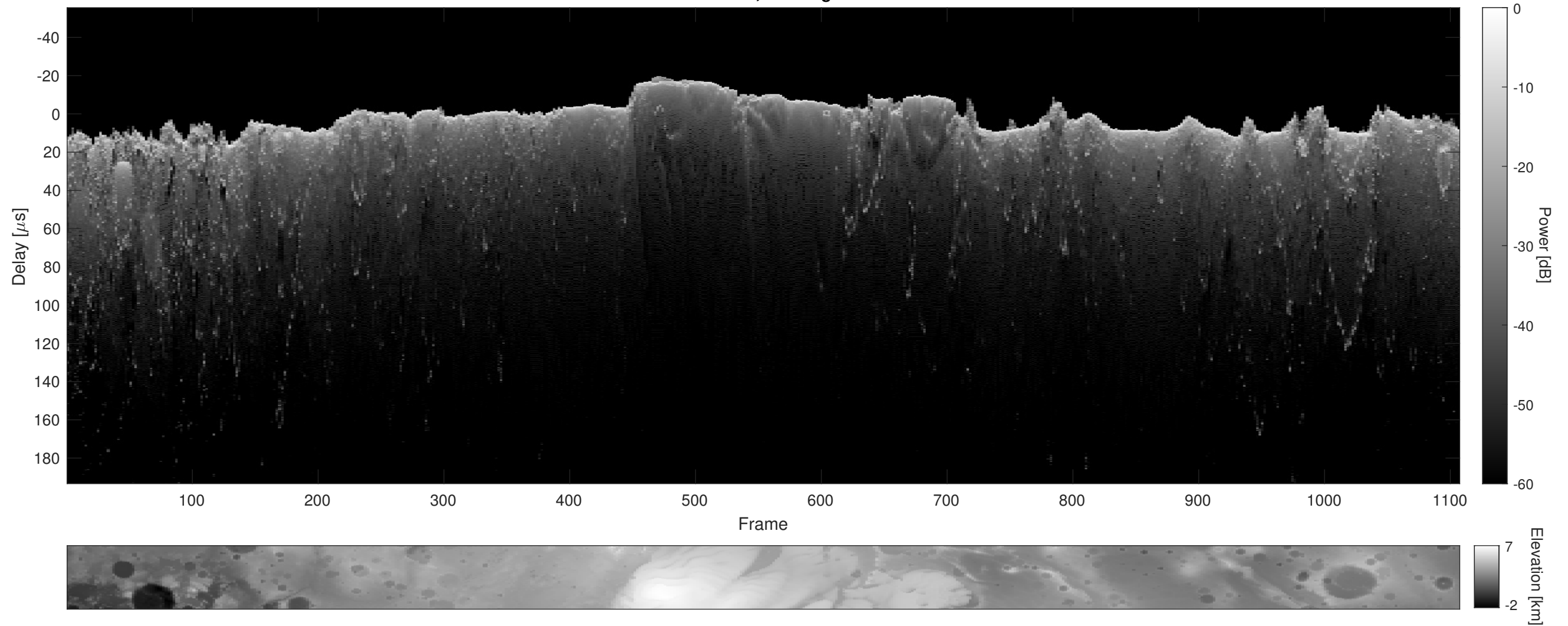
Orbit 10794, Cluttergram
