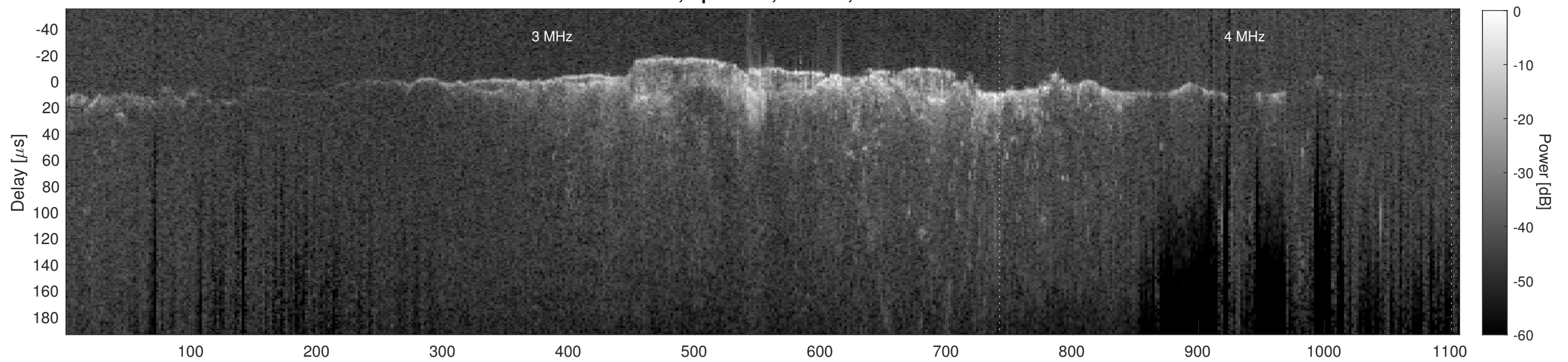
Orbit 10794, Cluttergram
