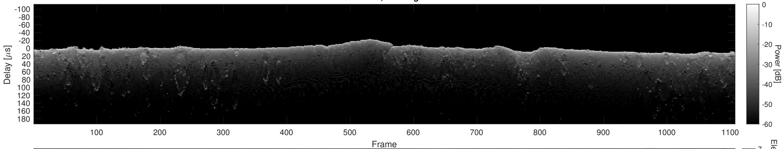
Orbit 10795, Cluttergram
