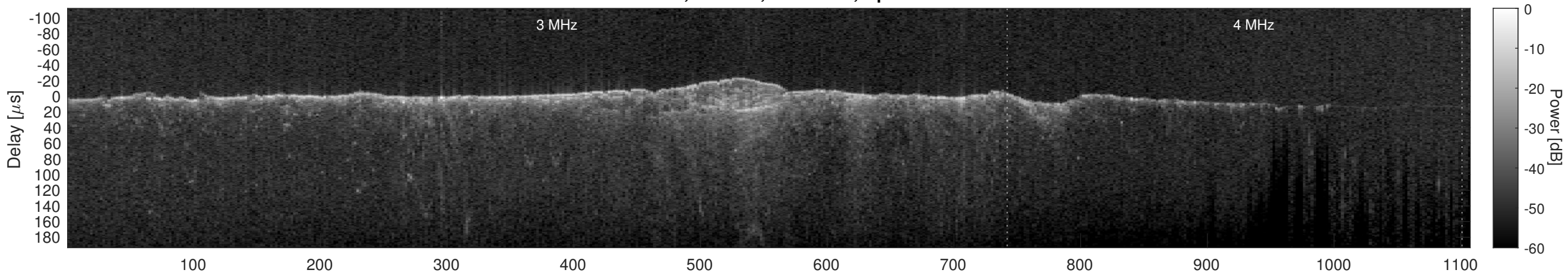
Orbit 10795, Cluttergram
