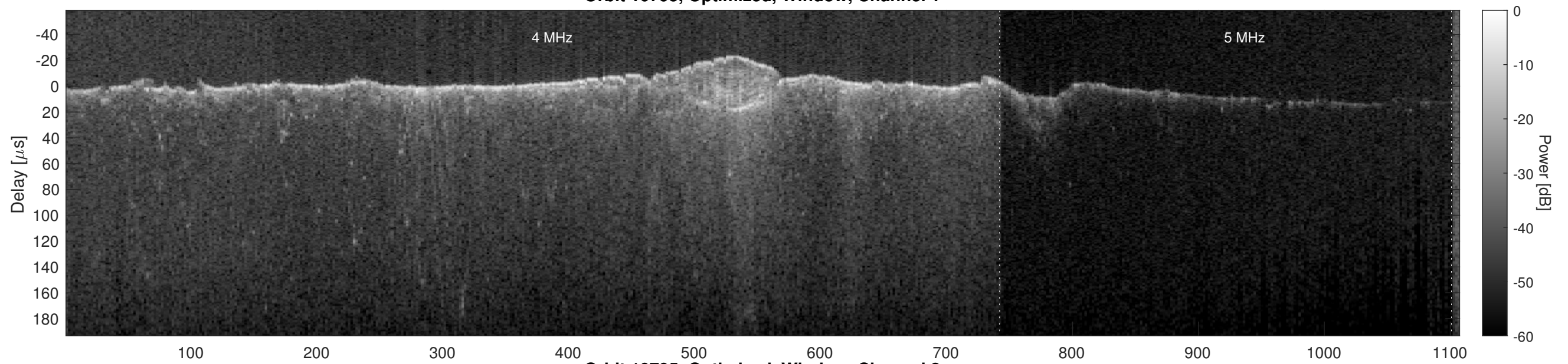
Orbit 10795, Optimized, Window, Channel 2
