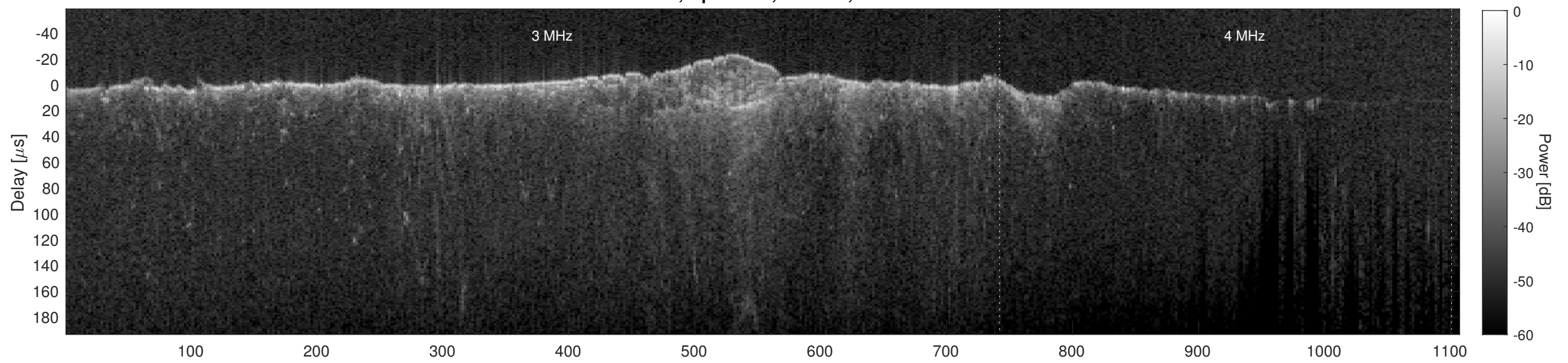
Orbit 10795, Cluttergram
