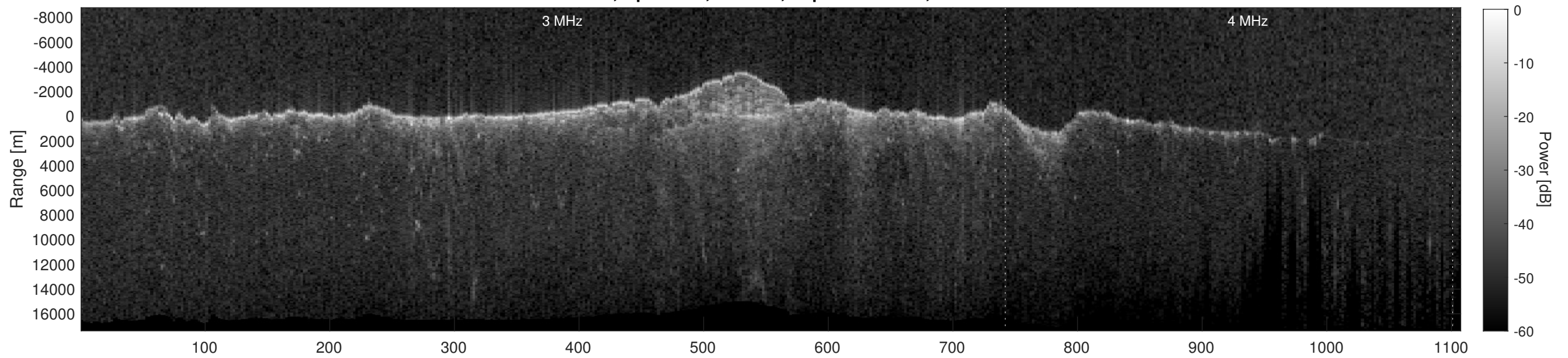
Orbit 10795, Depth-Corrected Cluttergram
