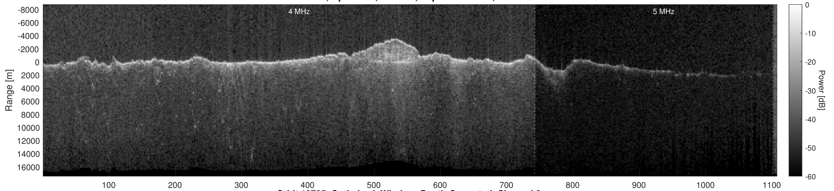
Orbit 10795, Optimized, Window, Depth-Corrected, Channel 2
