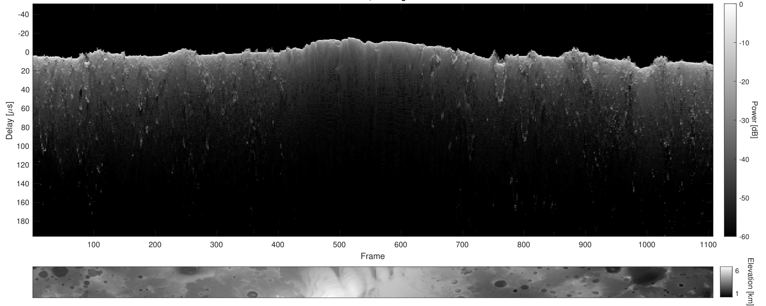
Orbit 10797, Cluttergram
