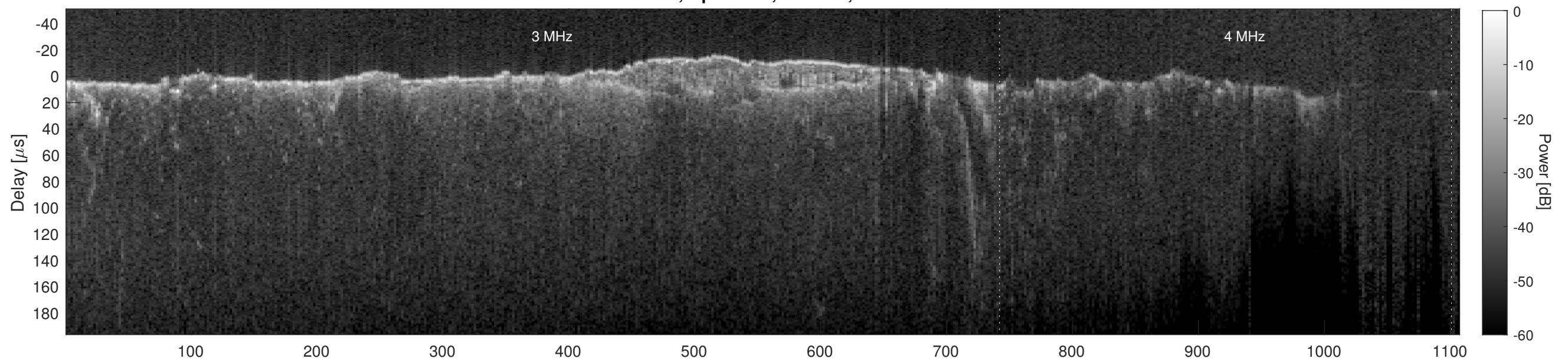
Orbit 10797, Cluttergram
