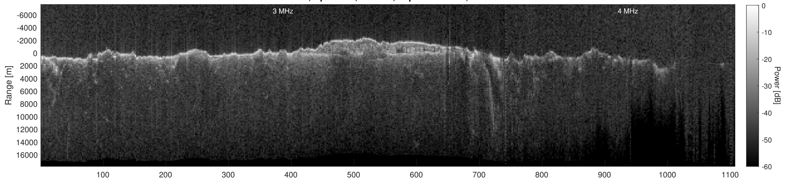
Orbit 10797, Depth-Corrected Cluttergram
