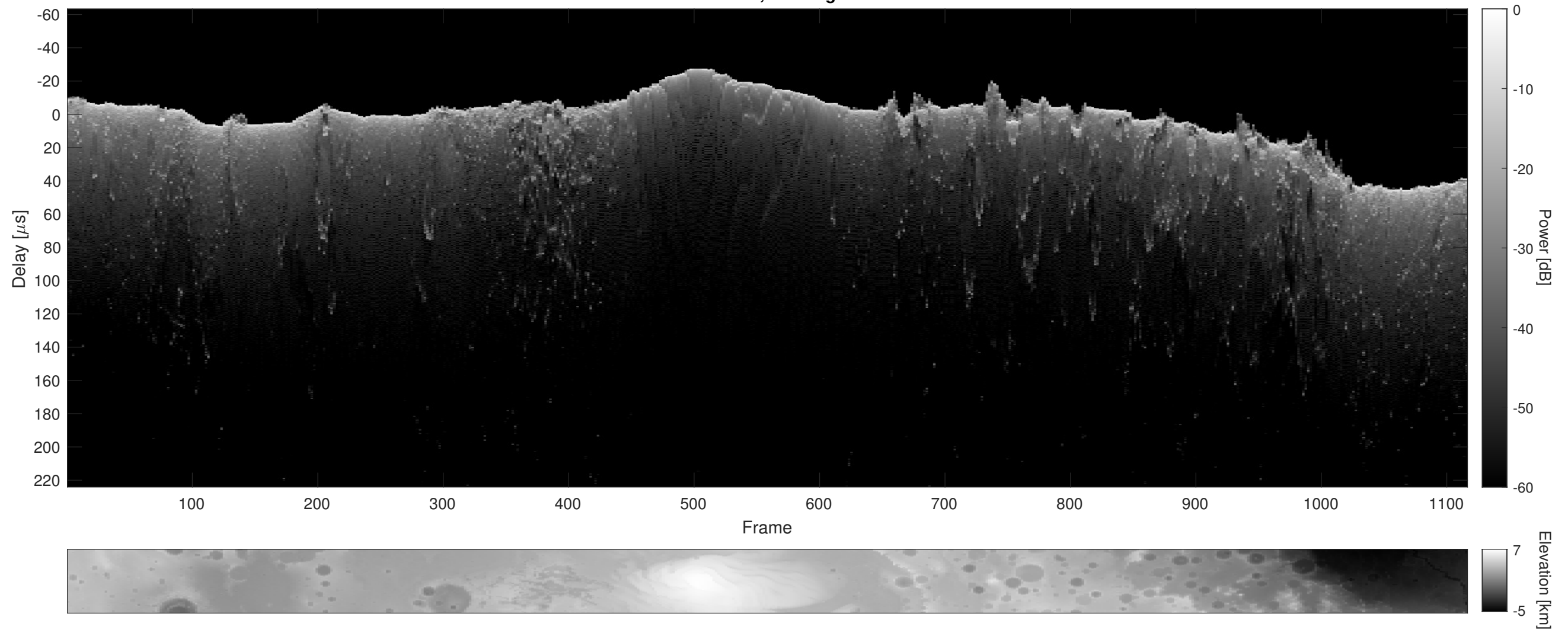
Orbit 10798, Cluttergram
