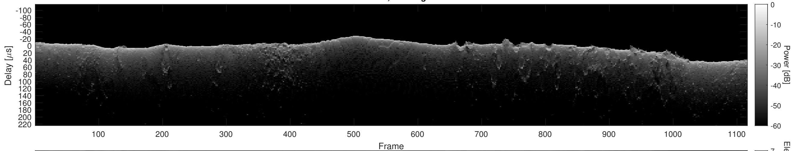
Orbit 10798, Cluttergram
