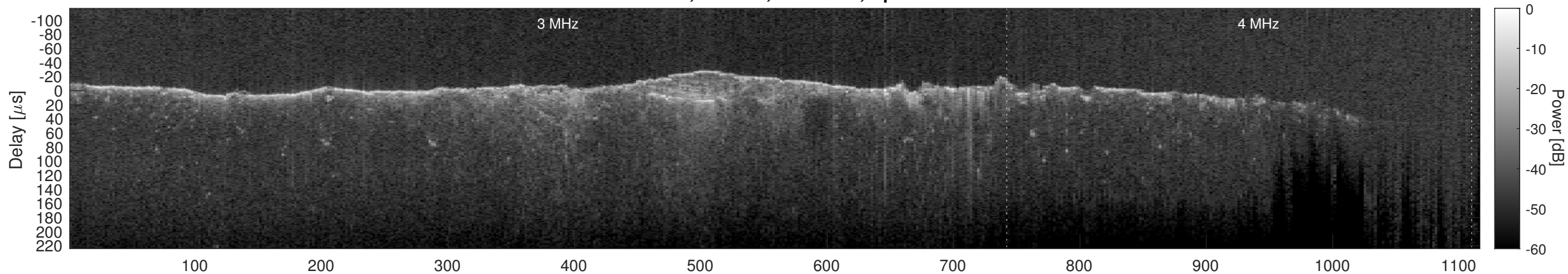
Orbit 10798, Cluttergram
