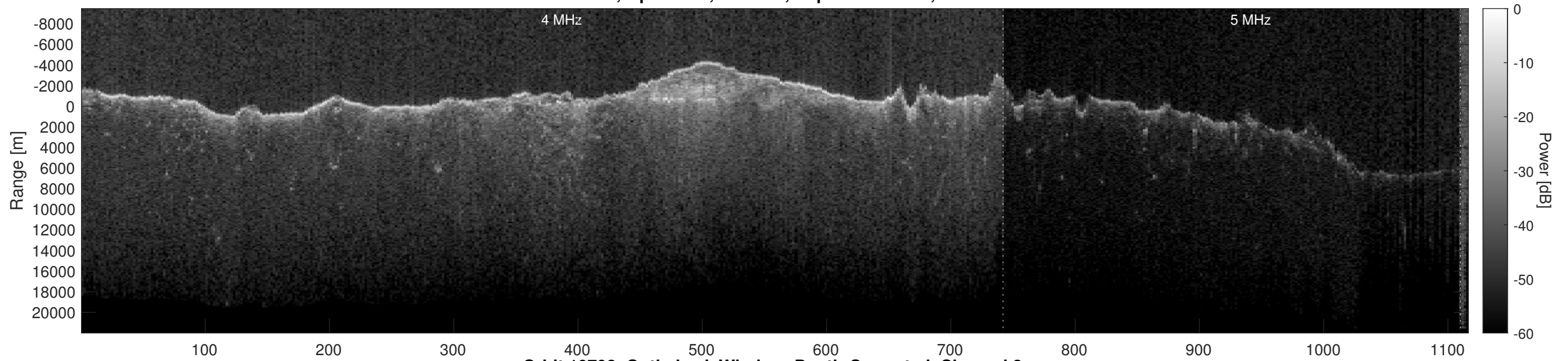
Orbit 10798, Optimized, Window, Depth-Corrected, Channel 2
