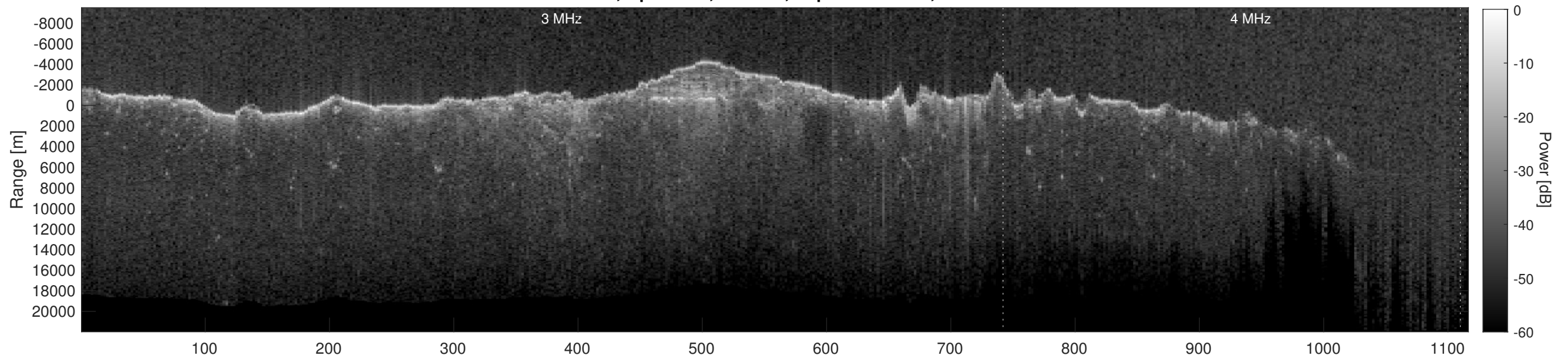
Orbit 10798, Depth-Corrected Cluttergram
