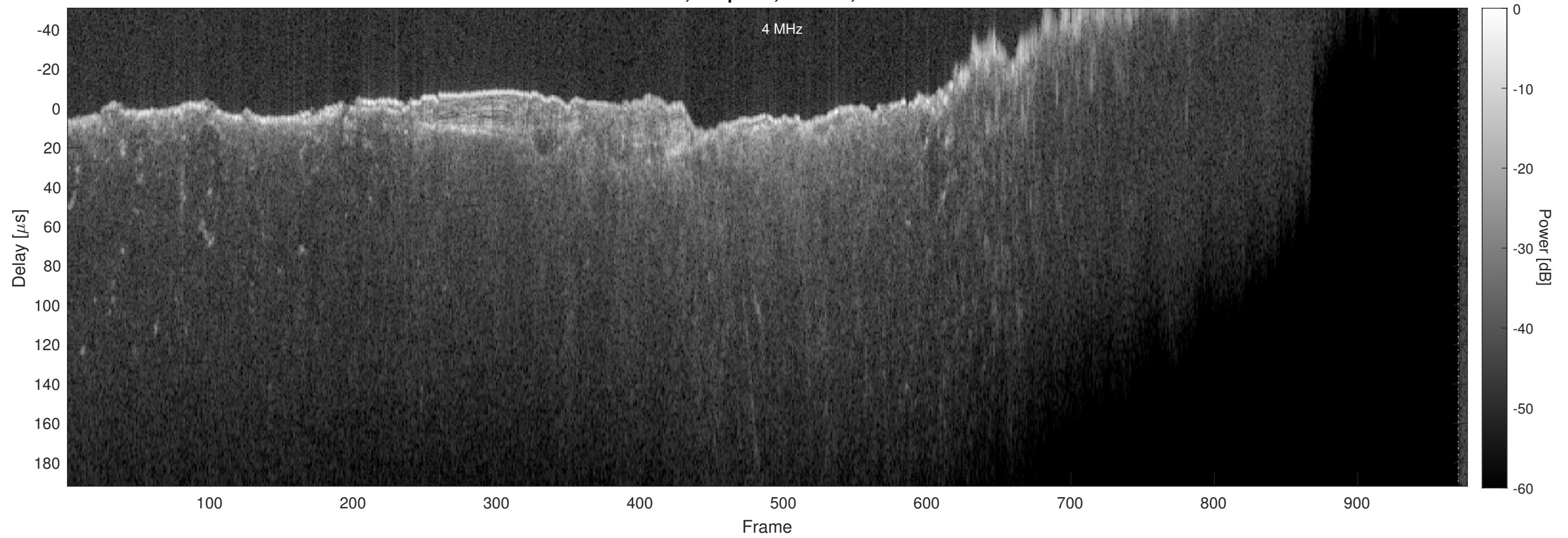
Orbit 10799, Chapman, Window, Channel 2
