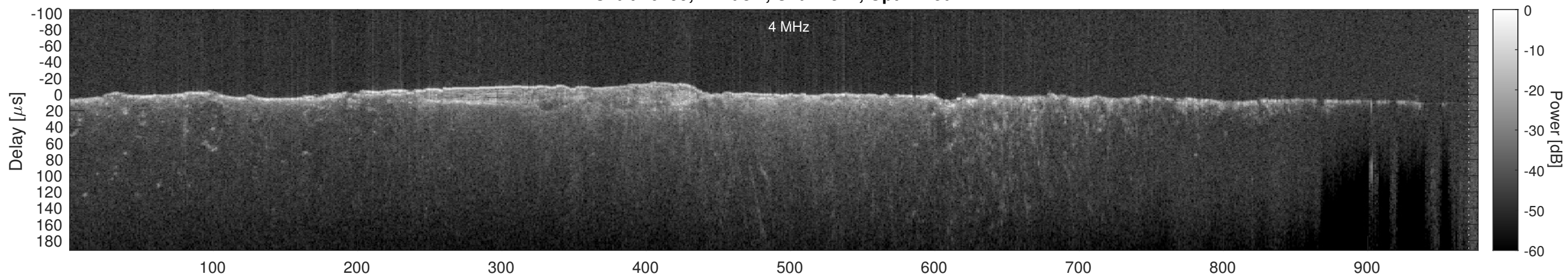
Orbit 10799, Cluttergram
