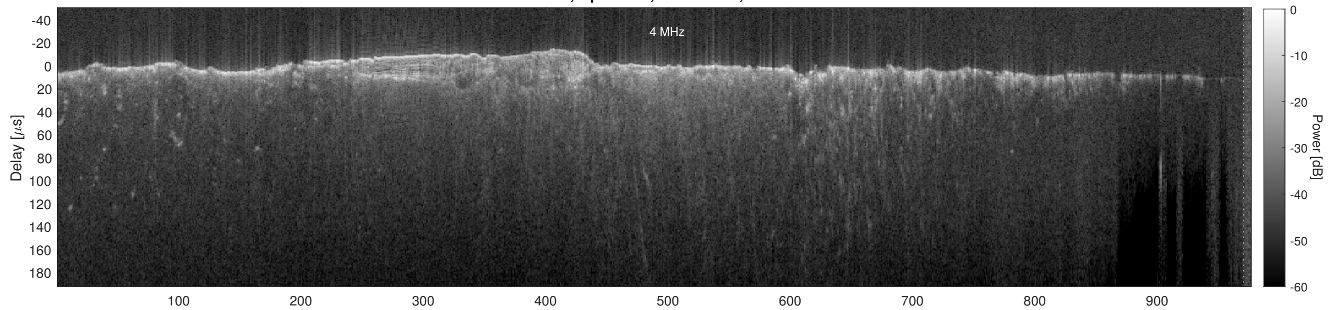
Orbit 10799, Cluttergram
