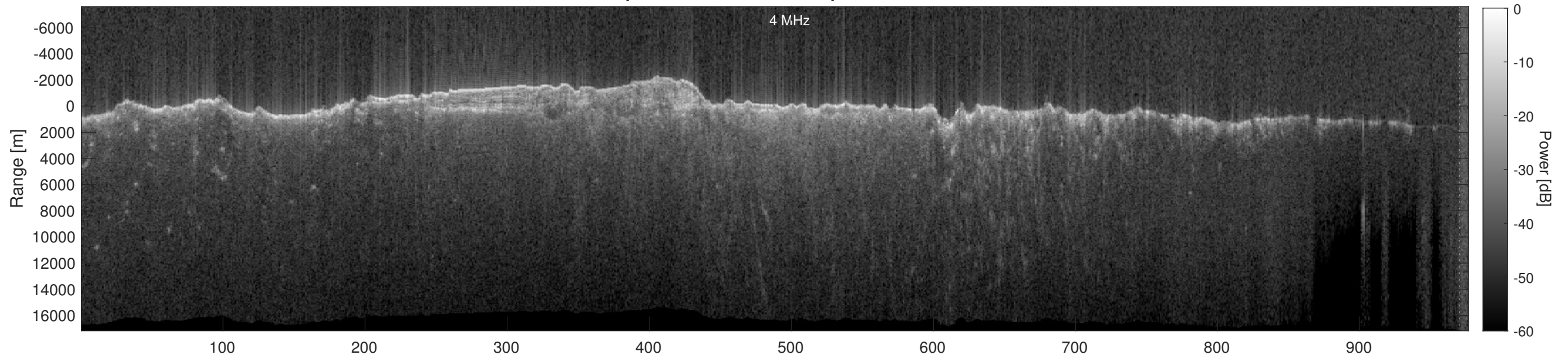
Orbit 10799, Depth-Corrected Cluttergram
