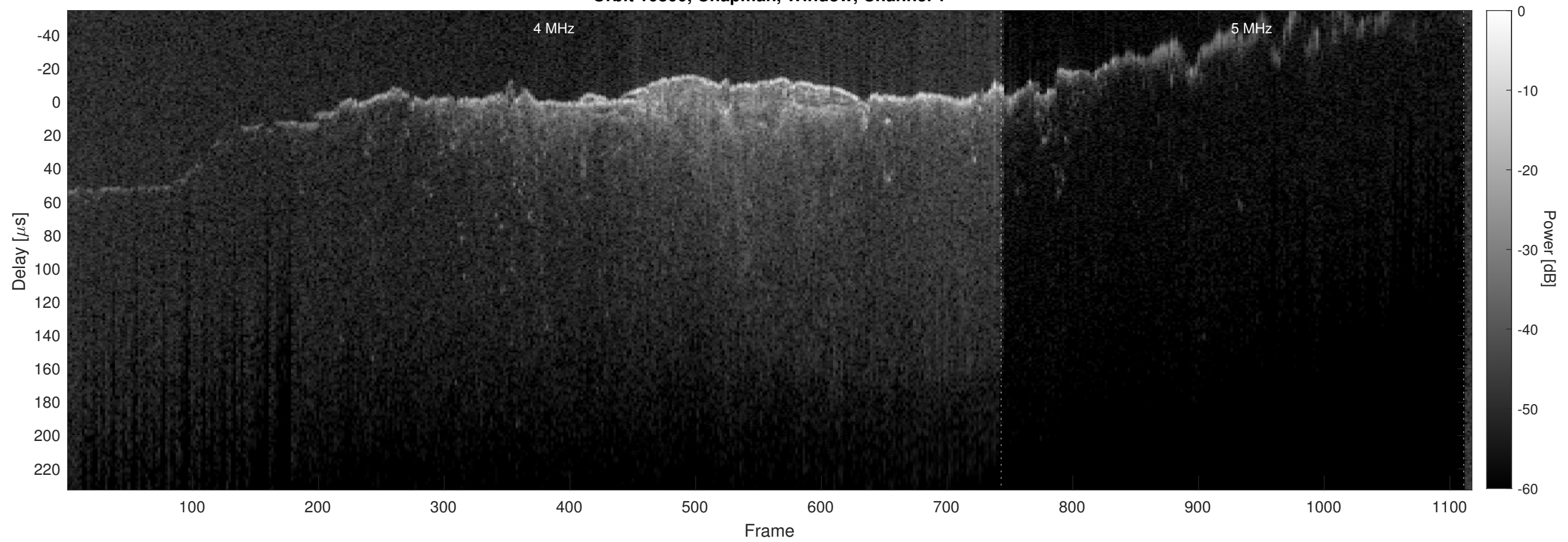
Orbit 10800, Chapman, Window, Channel 2
