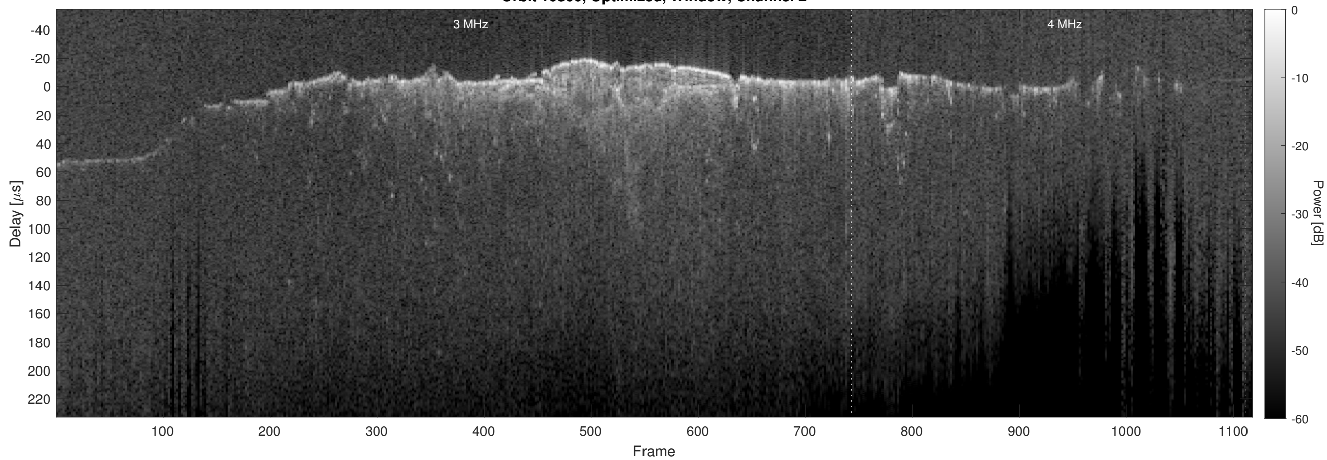
Orbit 10800, Optimized, Window, Channel 2
