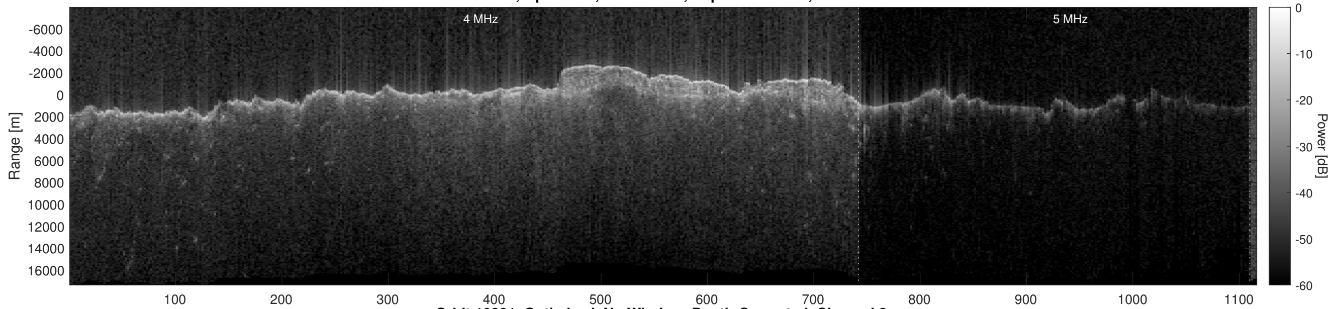
Orbit 10801, Optimized, No Window, Depth-Corrected, Channel 2
