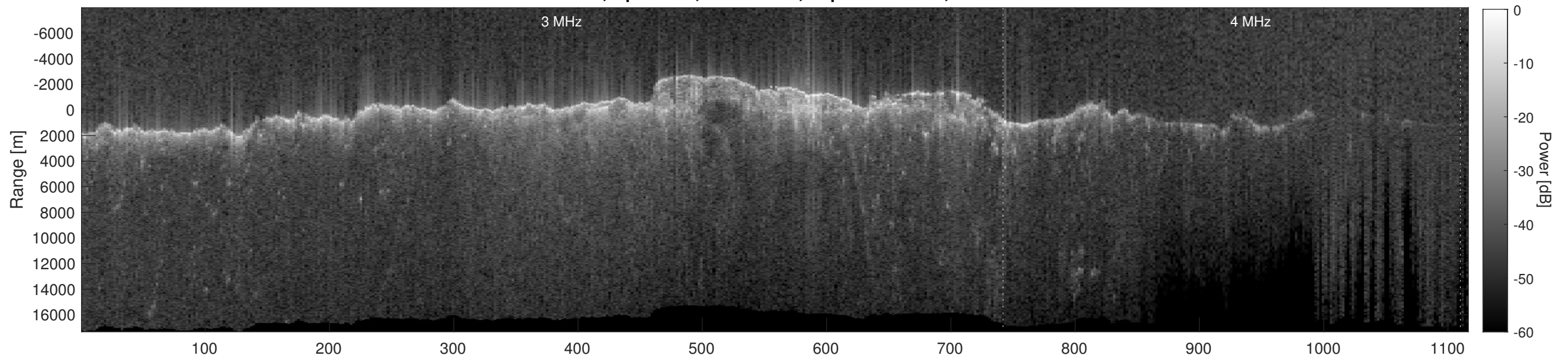
Orbit 10801, Depth-Corrected Cluttergram
